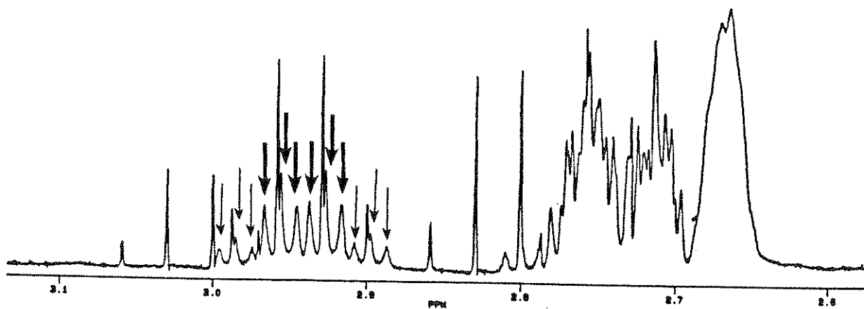
FIG 2. A portion of the 400 MHz 1 H NMR spectrum of the non-isolated mixture of the N -propionyl derivative 2 and its partially deuterated derivative 5.
